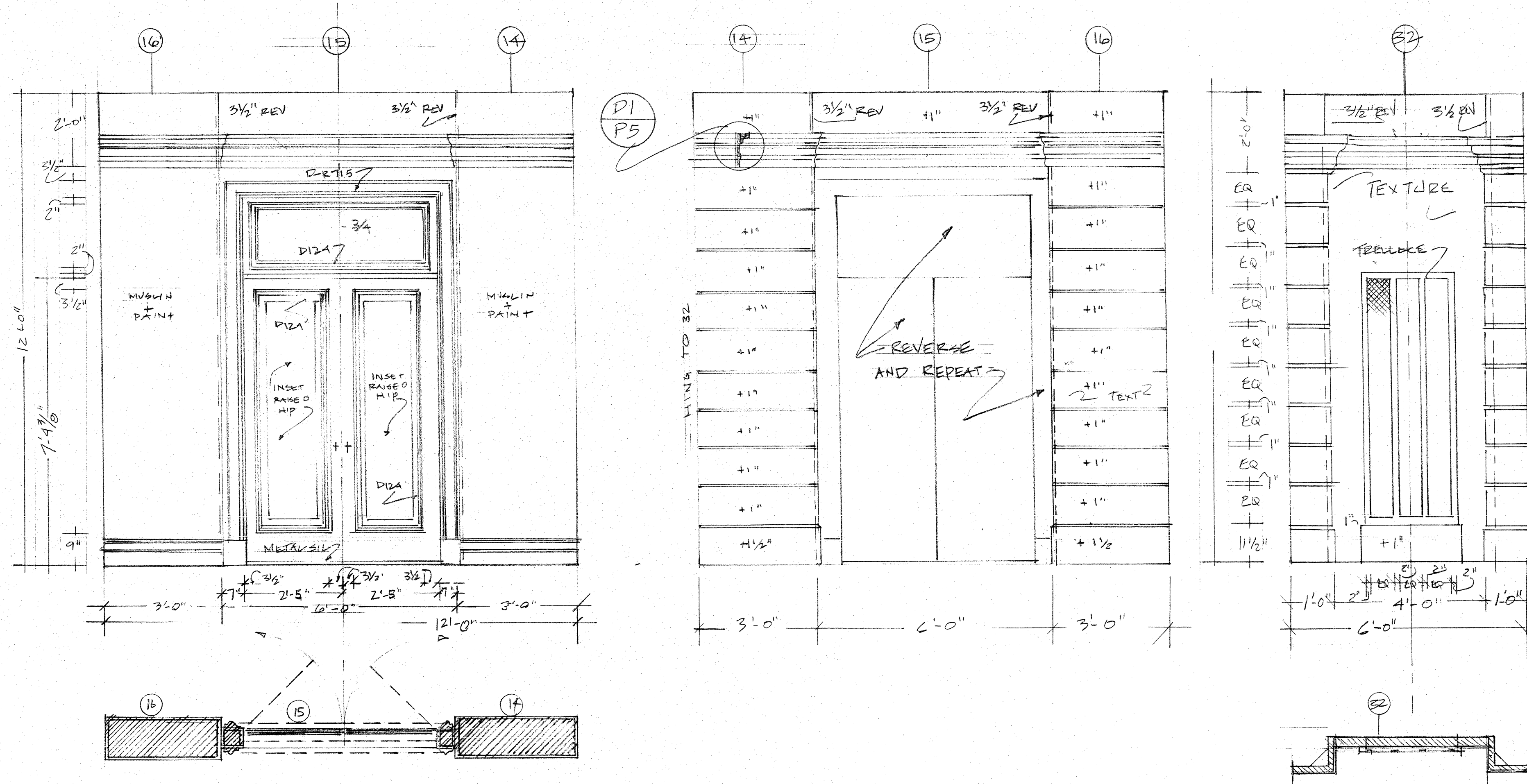
ENTRANCE DOORWAY SCALE 1/2" = 1'-0"
