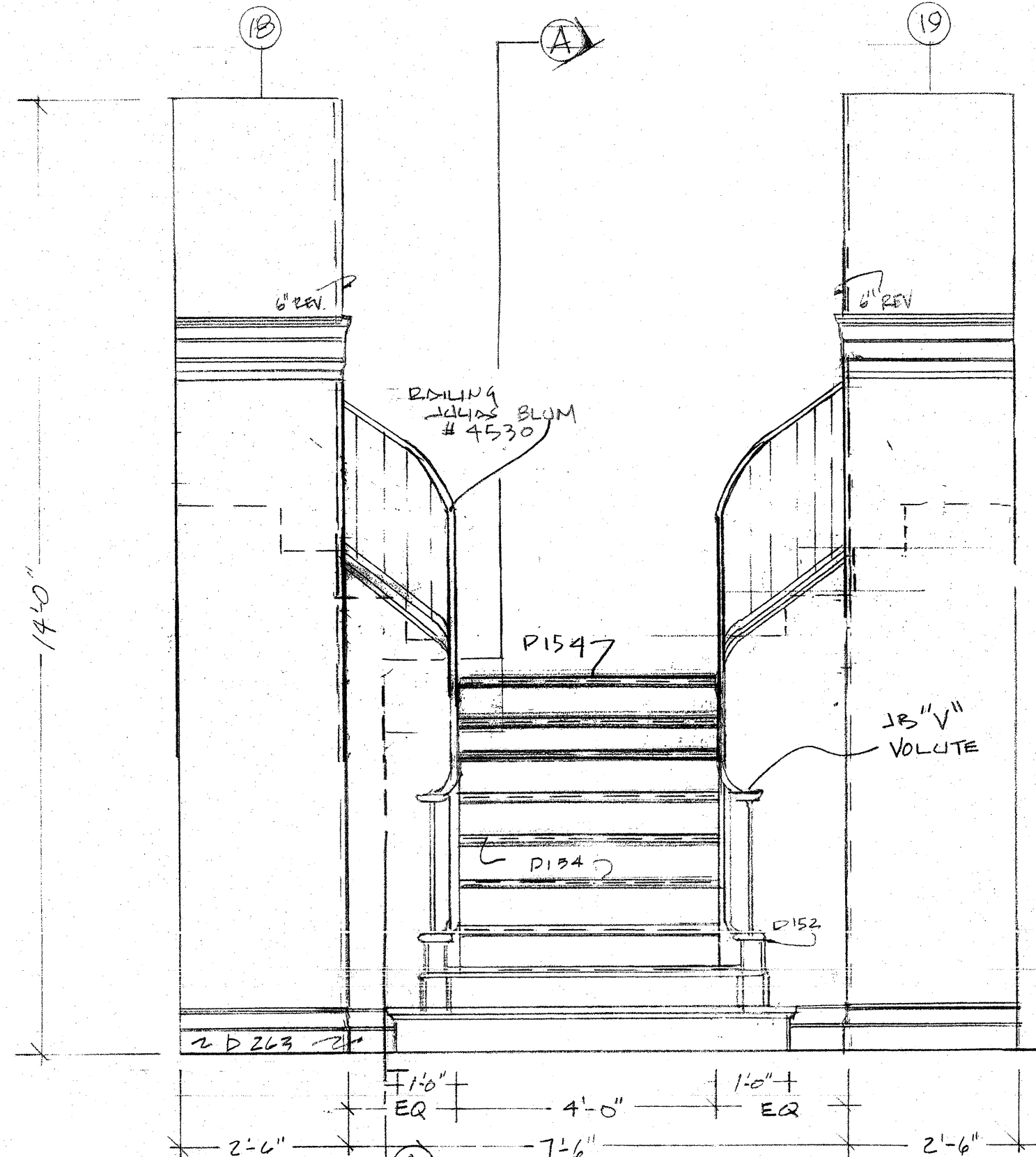
G. STAIRS SCALE 1/2" = 1'-0"
