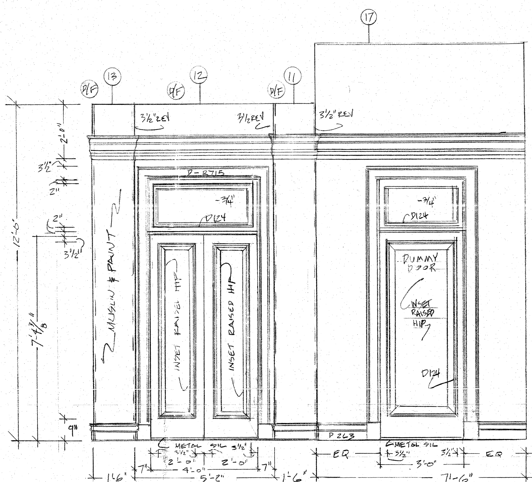
F. FRONT DOOR TO PARLOR SCALE 1/2" = 1'-0"
