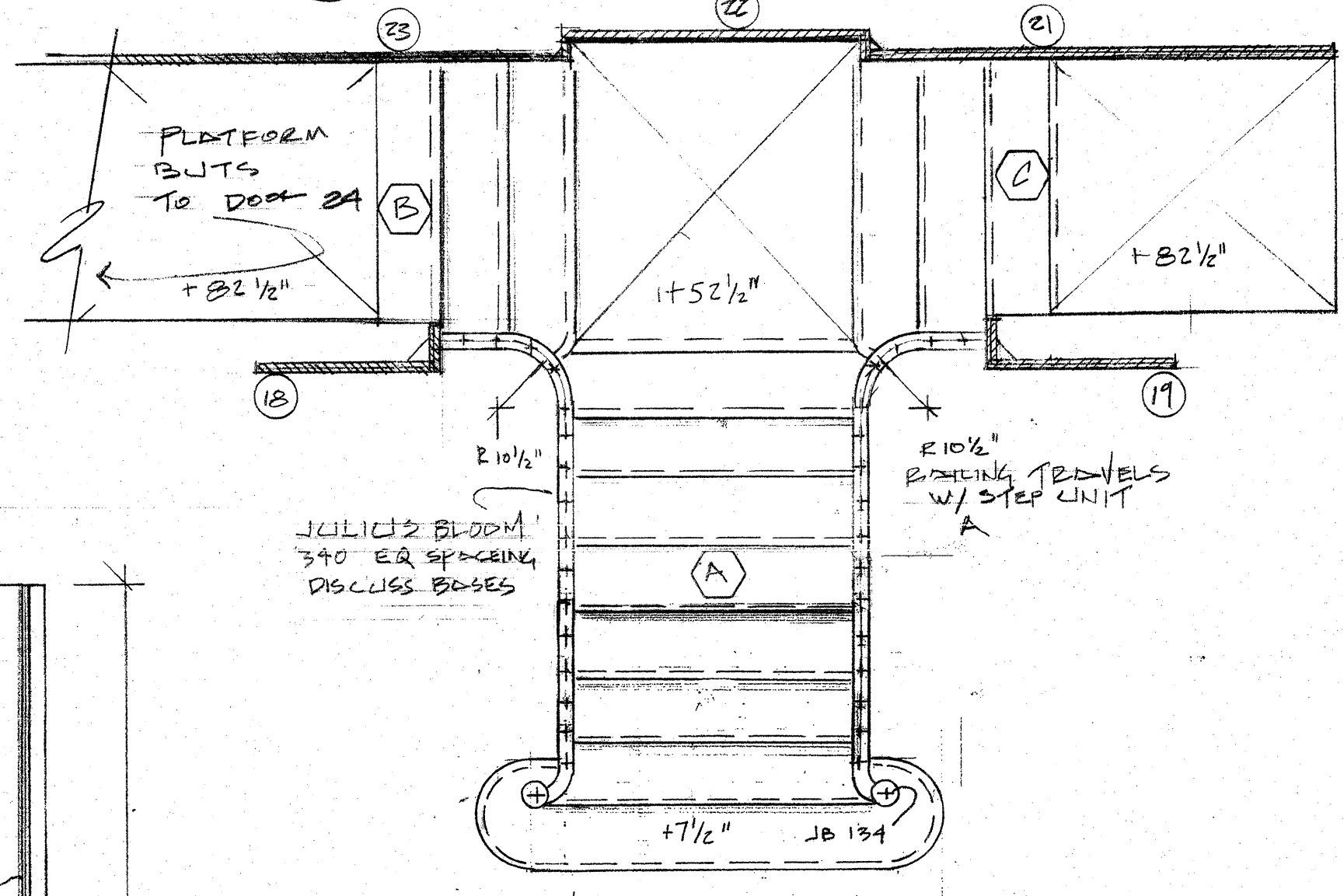
G. STAIRS SCALE 1/2" = 1'-0"
