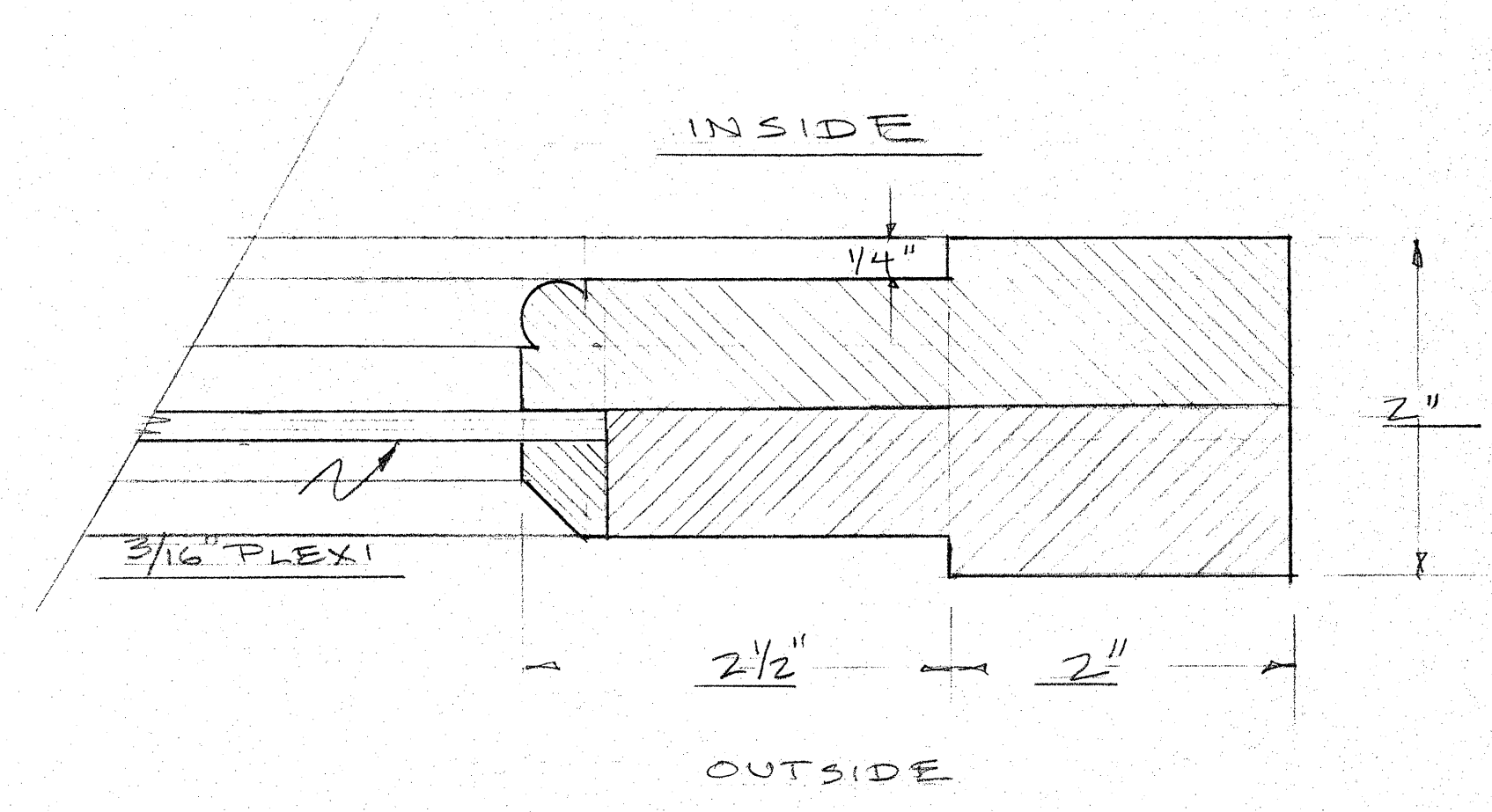
D3 DETAIL # 3 FULL SCALE OF DOORS
