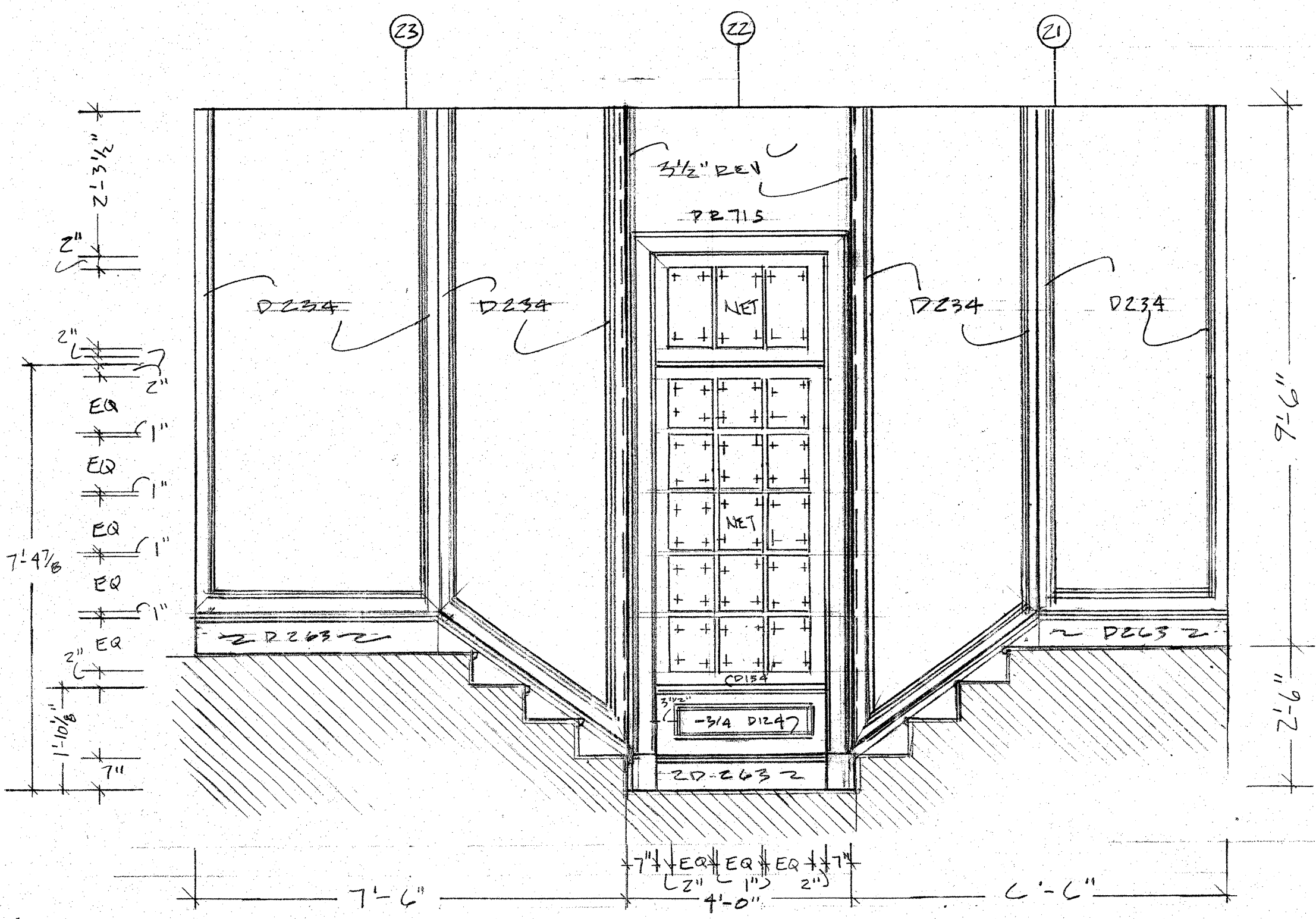
I. STAIR BACKINGS SCALE 1/2" = 1'-0"
