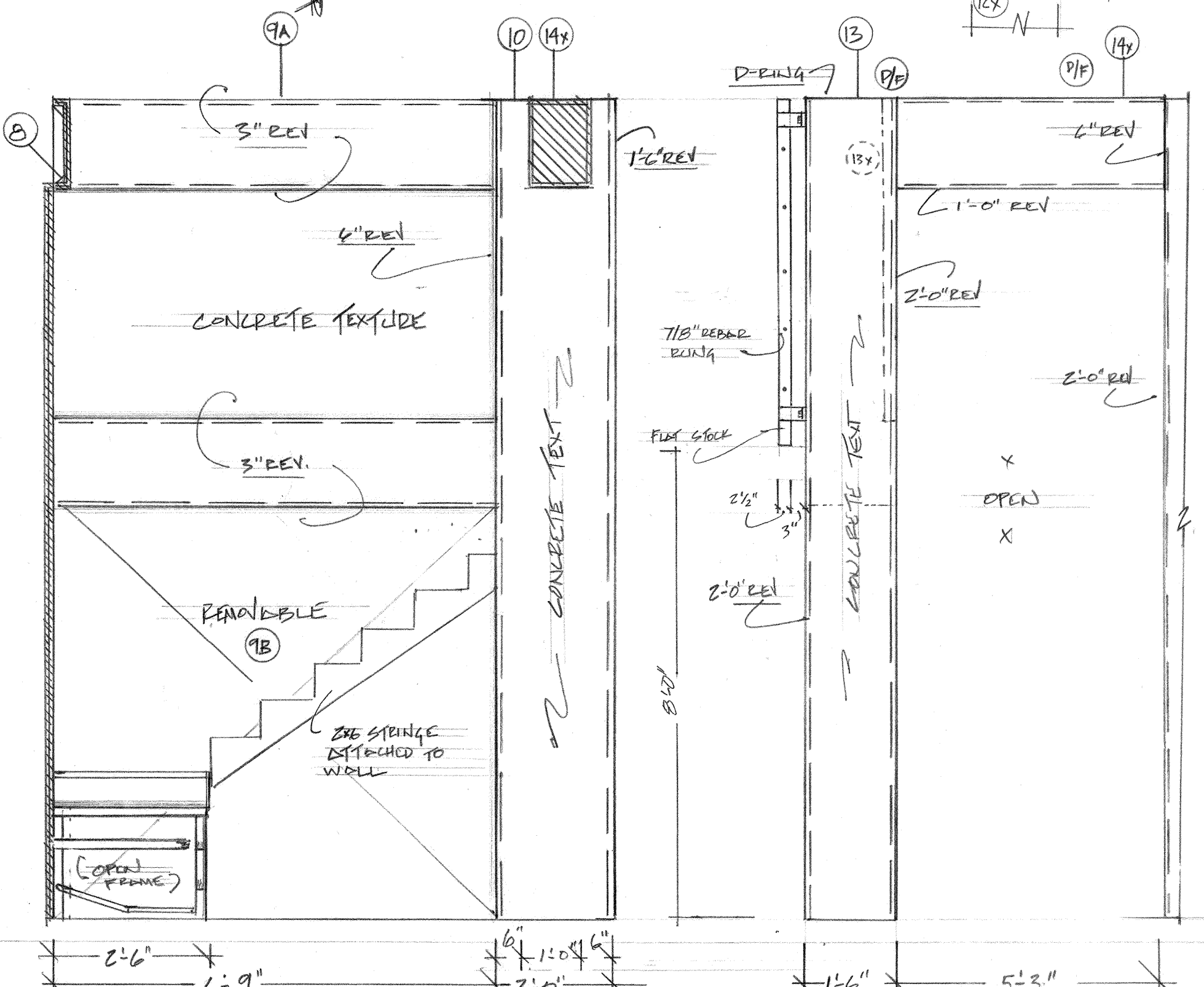
K SL WALL SCALE 1/2" = 1'-0"
