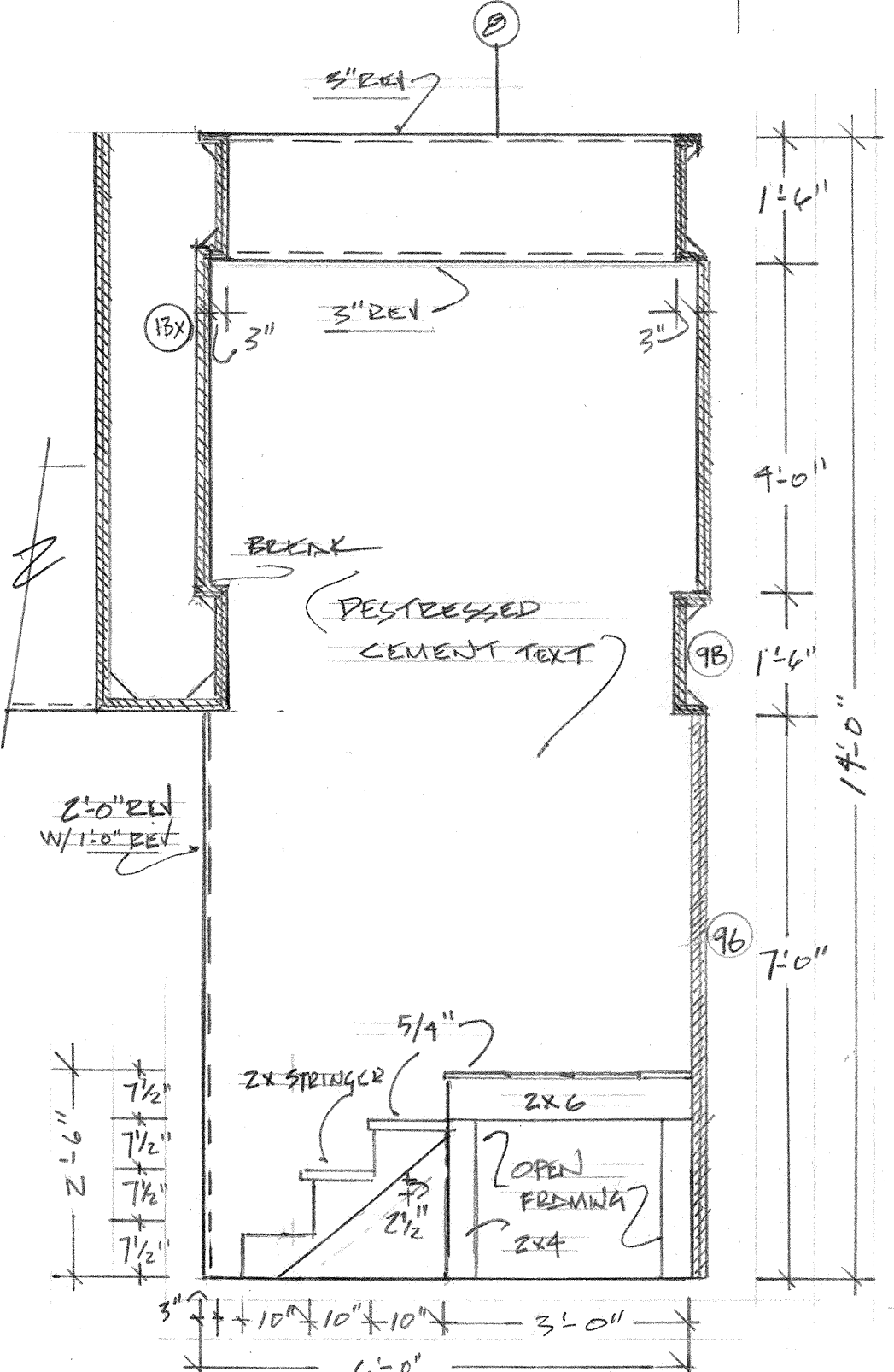
J SL ALCOVE SCALE 1/2" = 1'-0"
