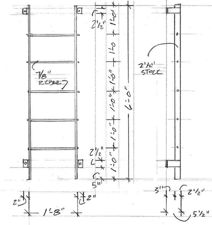
I PEBBLE LADDER SCALE 1/2" = 1'-0"
