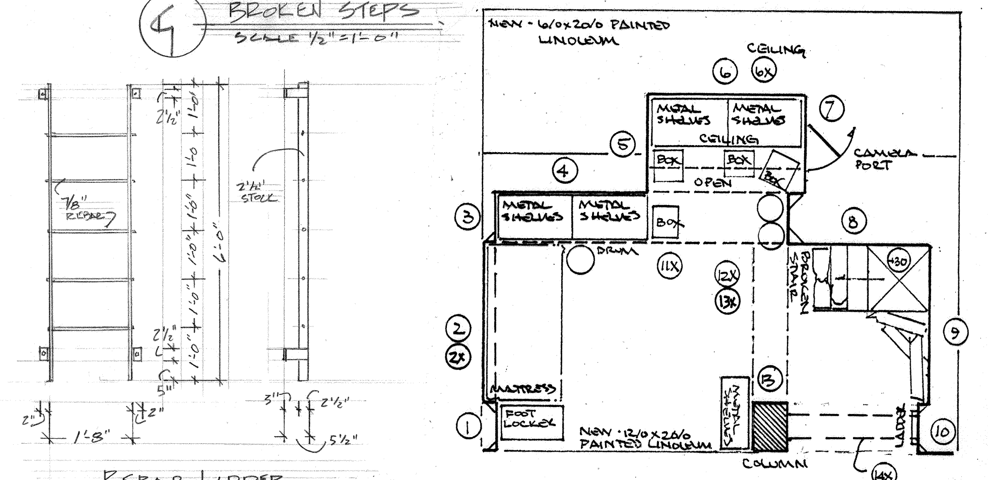
I PEBBLE LADDER SCALE 1/2" = 1'-0"
