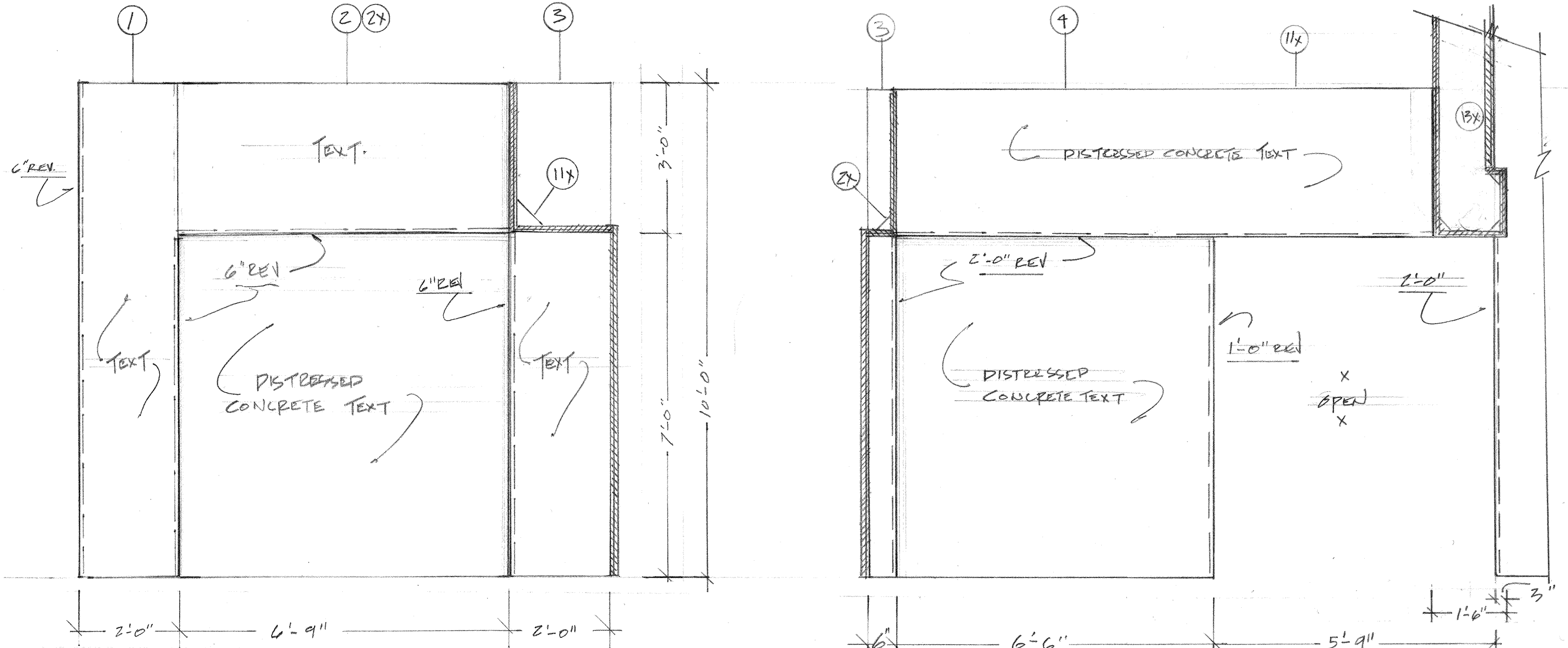
A DSR WALLS SCALE 1/2" = 1'-0"
