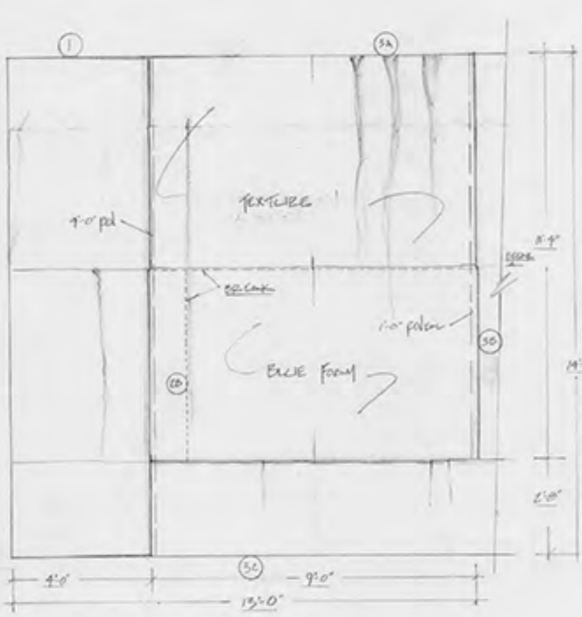
B DSR WALL SCALE 1/8"=1'-0"
