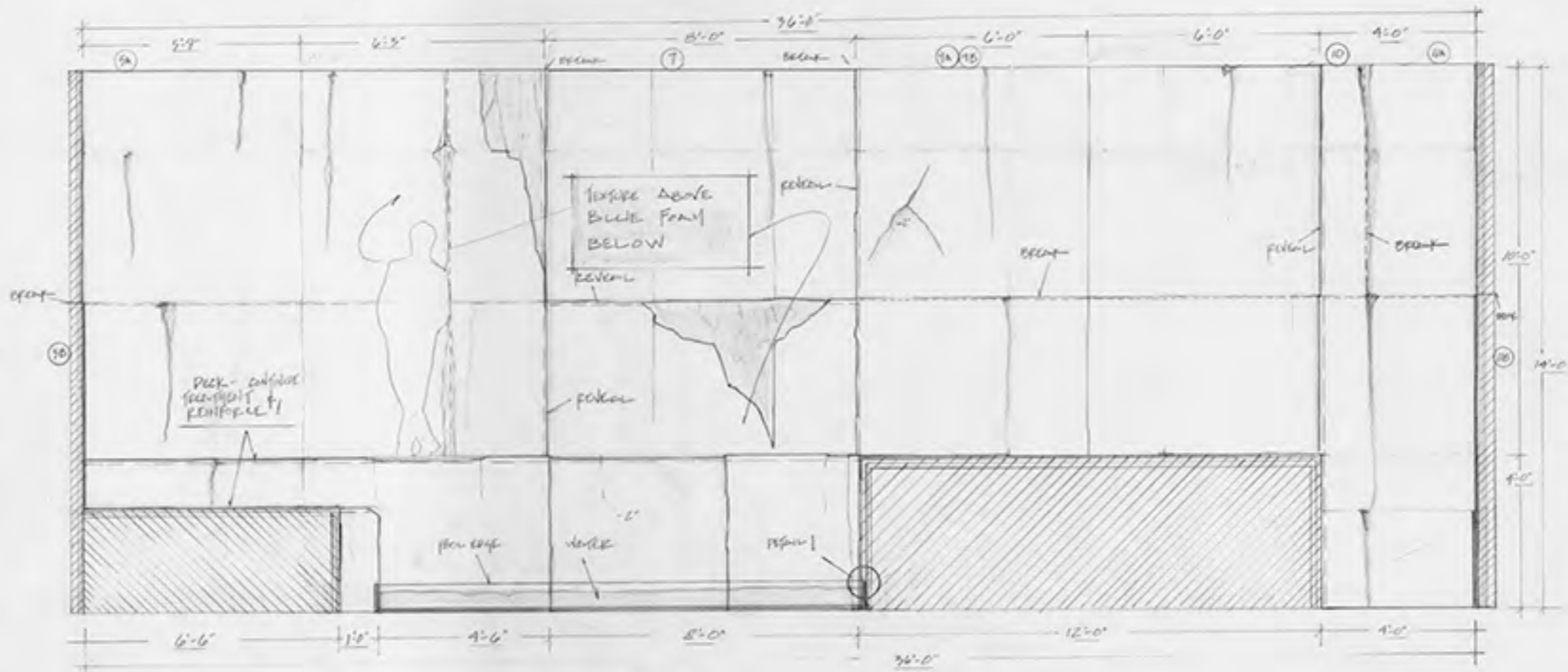
E USE WALL & POOL SCALE 1/2" = 1'-0"
