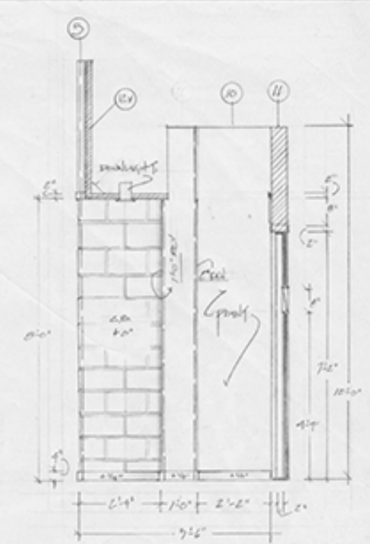
A-A SECTION A-A SCALE 1/2" = 1'-0"
