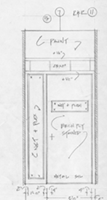
D. Close-up Door Detail FOR SCALE 1/2" = 1'-0"
