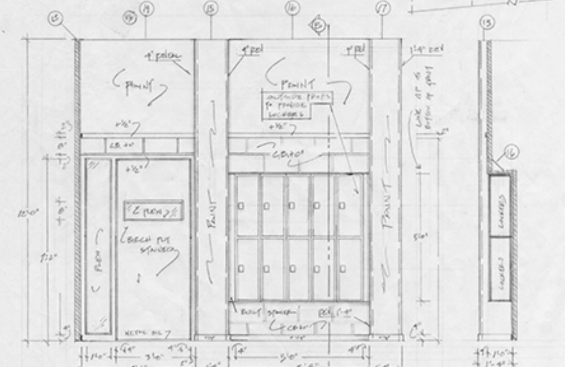
C. STAGE LEFT WALL SCALE 1/2" = 1'-0"
