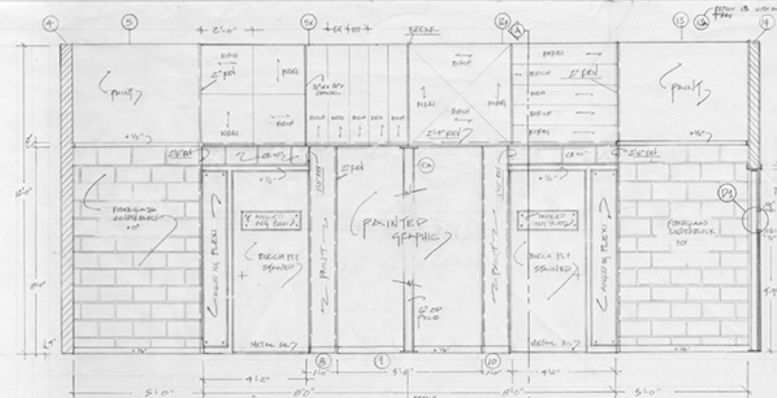
B. UP STAGE WALL SCALE 1/2" = 1'-0"
