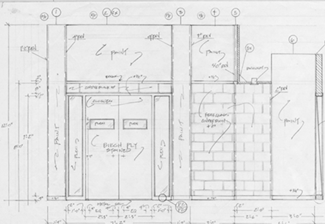
A. ENTRANCE SCALE 1/2" = 1'-0"
