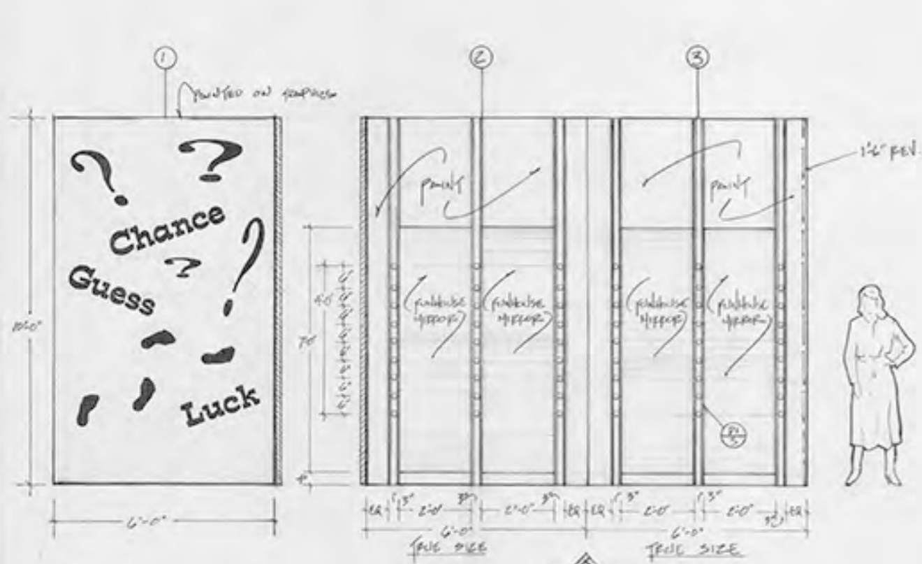
A WALL SCALE 1/2" = 1'-0"
