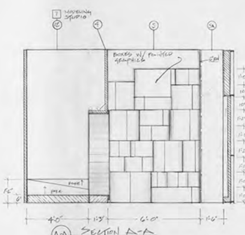
A-A SECTION A-A SCALE 1/2" = 1'-0"
